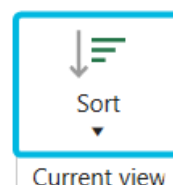
Figure 102. Button Sort
