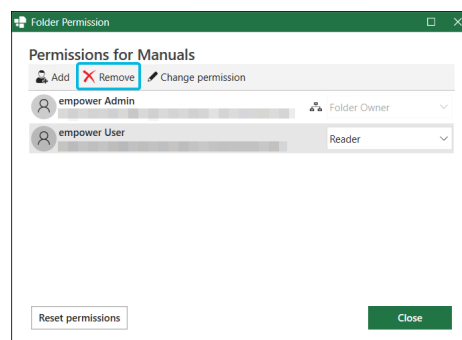
Figure 44. Button Remove
