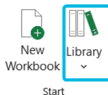
Figure 62. Button Library
