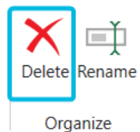
Figure 80. Button Delete
