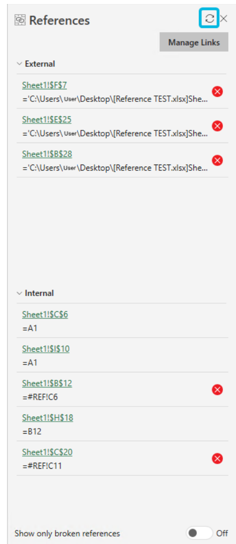
Figure 129. Refresh Symbol
