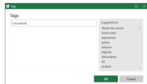
Figure 95. Window Tags
