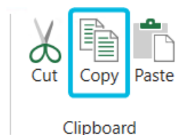
Figure 76. Button Copy
