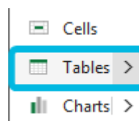
Figure 66. Option Tables
