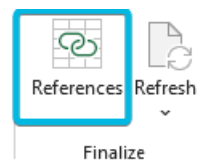
Figure 125. Button References
