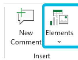
Figure 65. Button Elements
