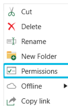
Figure 36. Option Permissions
