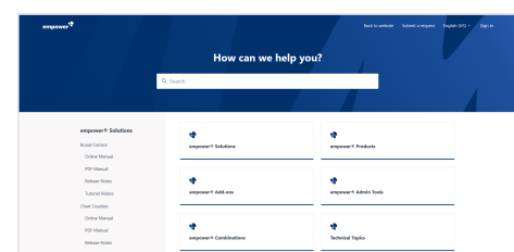
Figure 22. Help Center
