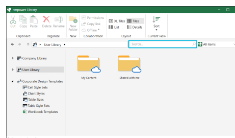
Figure 82. Search Bar
