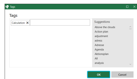
Figure 96. Button OK
