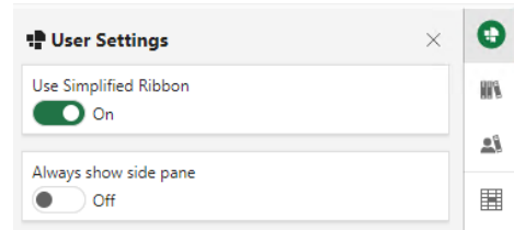
Figure 25. User Settings
