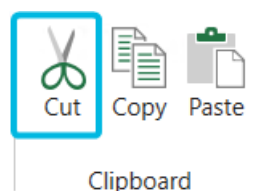
Figure 75. Button Cut
