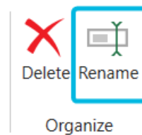
Figure 78. Button Rename
