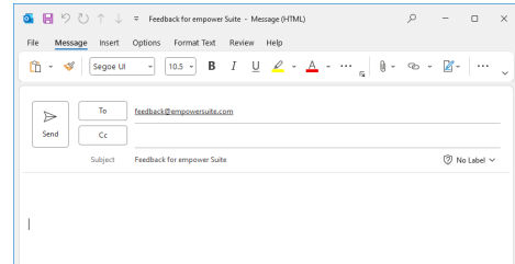
Figure 23. Feedback E-Mail
