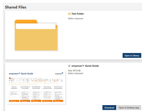
Figure 105. Shared Files
