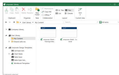
Figure 33. Library Window
