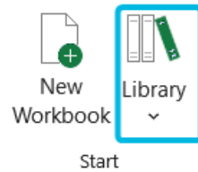
Figure 58. Button Library
