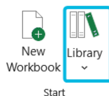
Figure 115. Button Library
