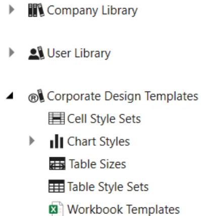
Figure 32. Library Structure
