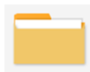
Figure 49. Offline Folder
