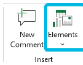
Figure 121. Button Elements
