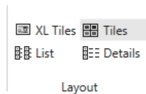
Figure 55. Group Layout
