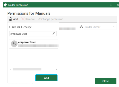
Figure 43. Button Add
