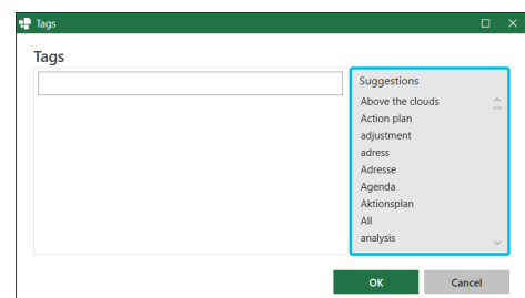
Figure 100. Tag List
