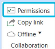
Figure 38. Button Permissions
