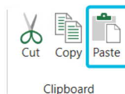
Figure 77. Button Paste
