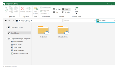
Figure 83. Search Scope
