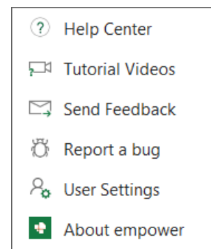
Figure 21. Help Options
